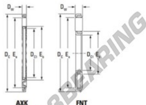
Boundary dimensions
